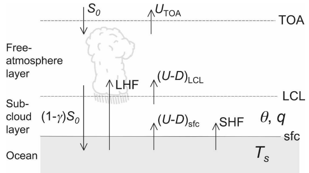
FIG. 1. Schematic diagram indicating the main variables, vertical layers, and energy fluxes considered in the model.
