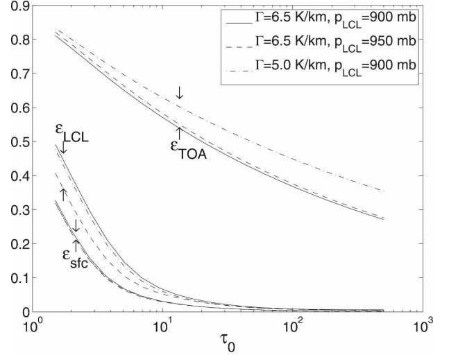
FIG. 4. Normalized net upward LW fluxes (for T_s = \theta ) at the surface ( \varepsilon_{\text{sfc}} ), LCL ( \varepsilon_{\text{LCL}} ), and TOA ( \varepsilon_{\text{TOA}} ) as a function of \tau_0 , for \Gamma = 6.5 \text{ K km}^{-1} and p_{\text{LCL}} = 900 \text{ hPa} (solid), \Gamma = 6.5 \text{ K km}^{-1} and p_{\text{LCL}} = 950 \text{ hPa} (dashed), and \Gamma = 5 \text{ K km}^{-1} and p_{\text{LCL}} = 900 \text{ hPa} (dotted-dashed).
