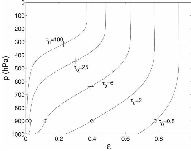
FIG. 3. Normalized vertical profiles of net upward LW fluxes \varepsilon(p, \tau_0, p_{\text{LCL}}, \Gamma) for different values of \tau_0 , with \Gamma = 6.5 \text{ K km}^{-1} , p_{\text{LCL}} = 900 \text{ hPa} (indicated with circles) and assuming T_s = \theta . The levels at which \tau = 1 are indicated with crosses.
