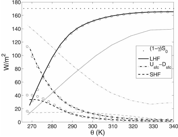
FIG. 5. Semianalytic solution for surface latent (solid), net long-wave (dotted-dashed), and sensible (dashed) heat fluxes vs surface air temperature using the semigray radiation for different values of \tau_0 (thick lines; the circles indicate results from the full model) and full radiative transfer with interactive water vapor feedback for different concentrations of \text{CO}_2 (thin lines). Both models have \Gamma = 6.5 \text{ K km}^{-1} and p_{\text{LCL}} = 900 \text{ hPa} .
