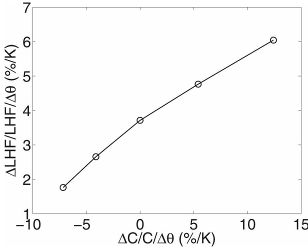
FIG. 7. Fractional changes in LHF per degree warming ( \% \text{ K}^{-1} ) for different changes in C ( \% \text{ K}^{-1} ).
