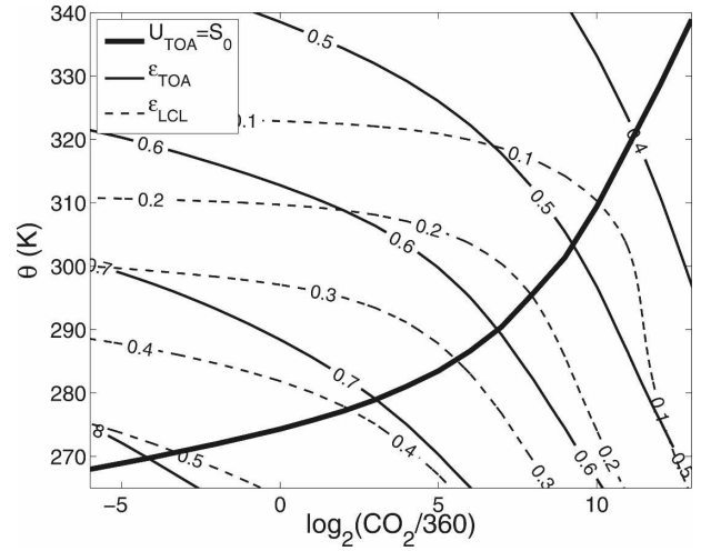
FIG. 8. Contours of \varepsilon_{\text{TOA}} (solid) and \varepsilon_{\text{LCL}} (dashed) as \text{CO}_2 concentration and water vapor are varied (the latter by changing \theta while keeping relative humidity constant). The thick curve denotes the states for which U_{\text{TOA}} = S_0 = 240 \text{ W m}^{-2} .
