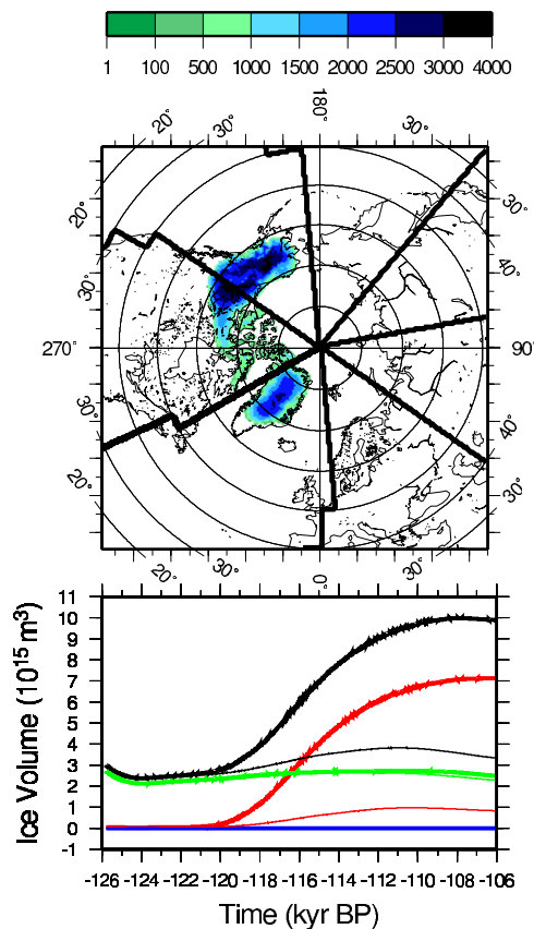
Figure 1. a. Final ice-sheet thickness (in m) in the ice-sheet model on the ISM grid ( 231 \times 241 points) and limits of the CLIMBER sectors (thick lines in longitude, thin parallels for latitudinal boundaries); b. evolution of the volume (in \text{Pm}^3 ) of the main NH ice-sheets simulated by the model forced by the insolation and \text{CO}_2 of the period 126–106 kyr BP: total volume (black), Greenland (green), Laurentide (red), Fennoscandia (blue); thin lines are for experiment with vegetation fixed at its initial value.
