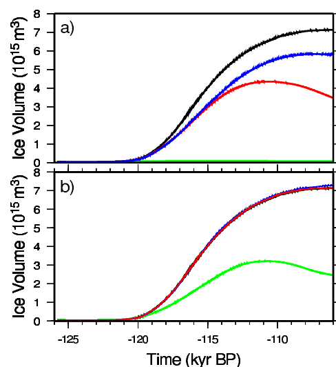
Figure 3. North American ice volume in 126–106 ky BP runs all forced by the same insolation and \text{CO}_2 as the STD run (in black), but with one coupling variable fixed after 122 ky BP. a) sensitivity to variables passed from CLIMBER to the ISM: green: fixed \text{Tjja} , red: fixed \text{Tann} , blue: fixed \text{Snw} ; b) sensitivity to the variables passed from the ISM to CLIMBER: green: fixed glaciers' extent. The curves for STD (black), fixed glacier altitude (blue) and no correction in the fresh water going to the ocean (red) are superimposed.
