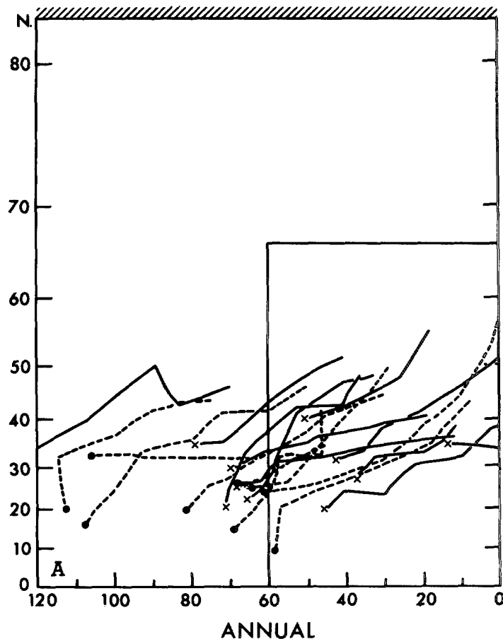
FIGURE 54.—Horizontal distribution of the conversion of available potential energy into kinetic energy due to transient eddies, that is,
