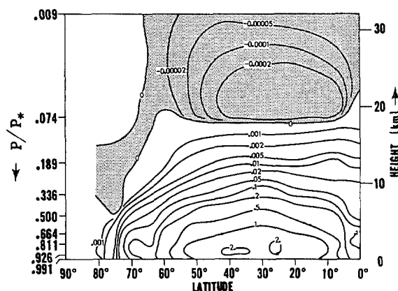
FIGURE 29.—Latitude-height distribution of poleward transport of water vapor by transient eddies in the model atmosphere (units, 10^{14} gm mb ^{-1} day ^{-1} ). The distributions of the two hemispheres are averaged.
