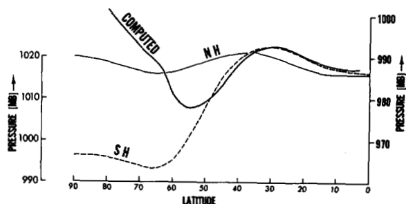
FIGURE 8.—Latitudinal distributions of the zonal mean surface pressure. The scale for the observed distributions is shown on the left ordinate and the scale for the computed distribution is shown on the right ordinate. The observed distributions for the Northern and Southern Hemispheres are indicated by NH and SH, respectively. The computed distribution is obtained by taking the average of the two hemispheres.
