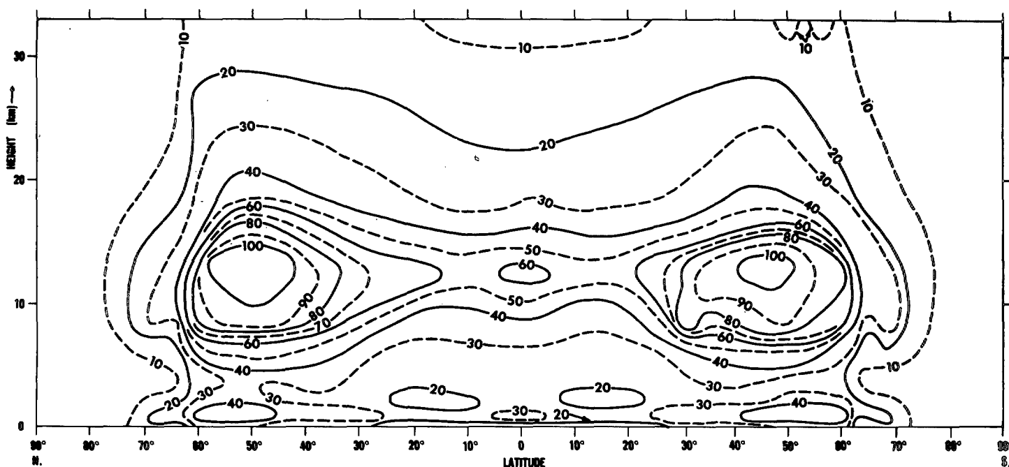
FIGURE 50.—Latitude-height distribution of the zonal mean eddy kinetic energy in the model atmosphere (units, joules cm -2 mb -1 ).
