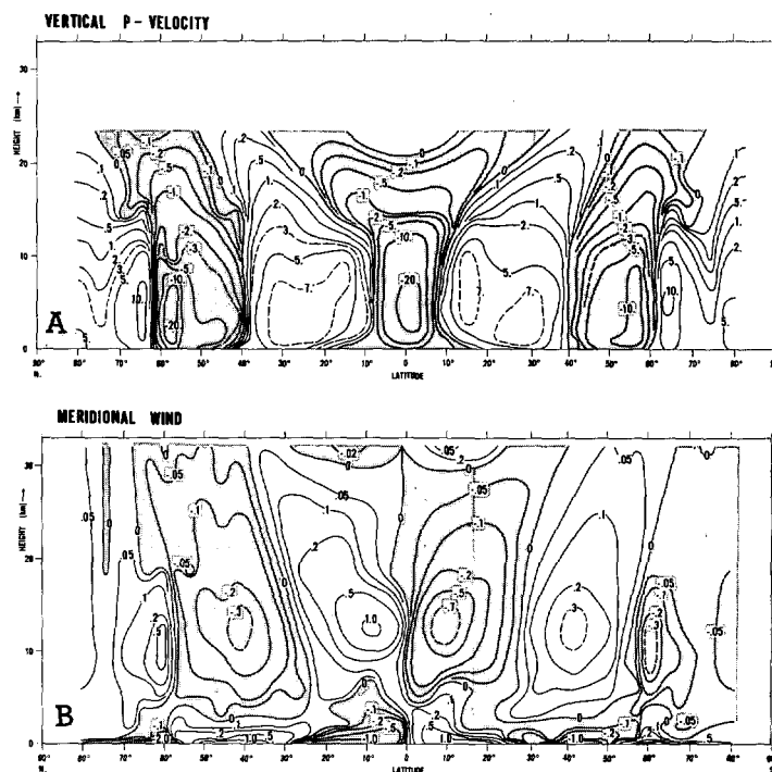
FIGURE 11.—Latitude-height distribution in the model atmosphere of (A) the zonal mean of the vertical P -velocity ( \text{mb day}^{-1} ) and (B) the zonal mean of the meridional component of the wind ( \text{m sec}^{-1} ). The regions of upward or southward components of wind are shaded.
