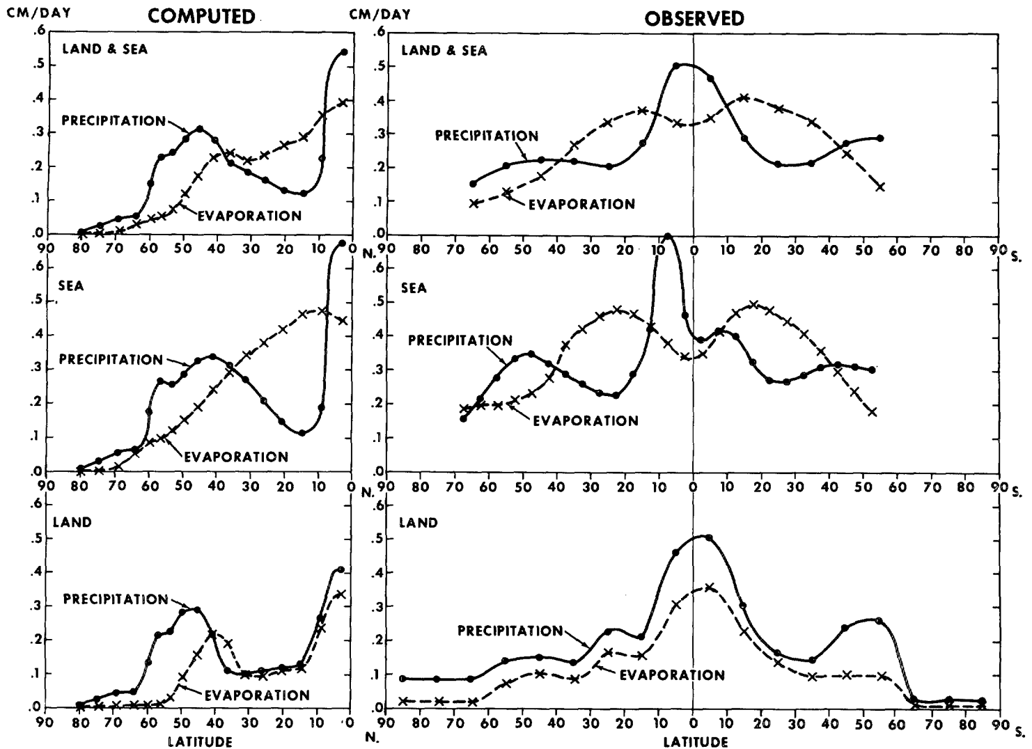
FIGURE 23.—Latitudinal distributions (computed and observed) of zonal mean precipitation and evaporation; the distribution of the model (computed) is obtained by taking the average of the two hemispheres.
