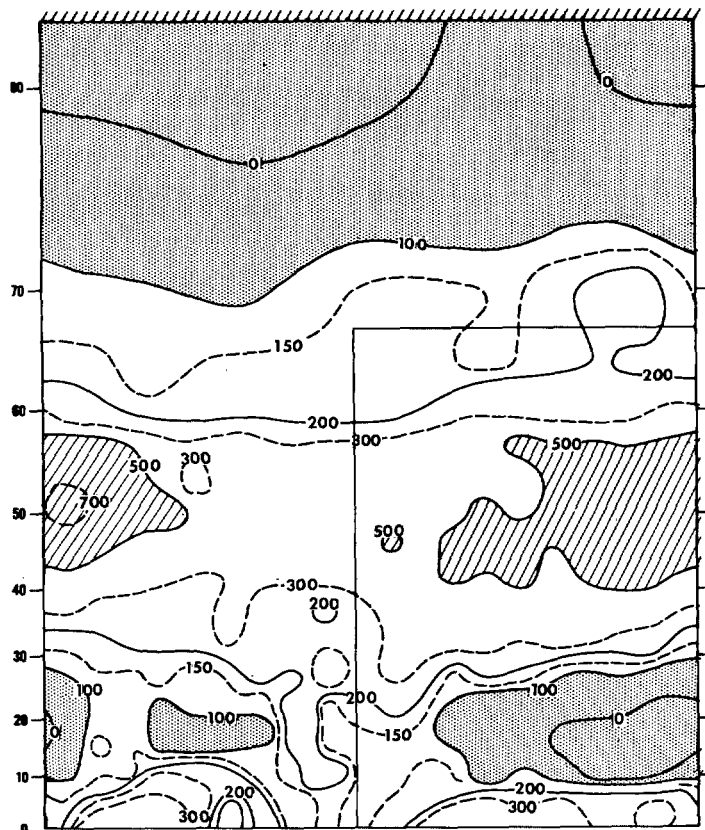
FIGURE 54.—Horizontal distribution of the conversion of available potential energy into kinetic energy due to transient eddies, that is,
