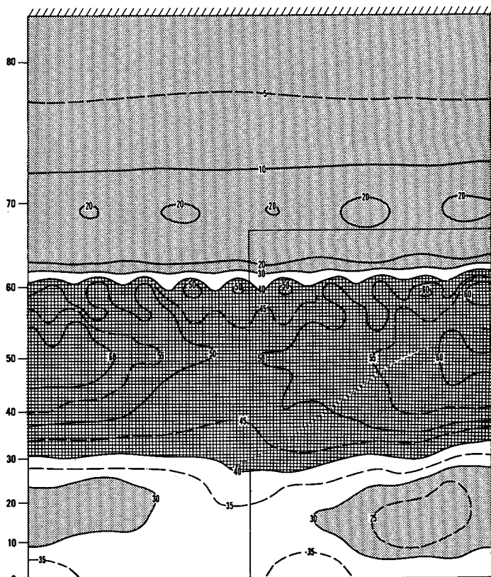
FIGURE 52.—Horizontal distribution of the vertical integral of eddy kinetic energy in the model atmosphere (average of two hemispheric values); units, joules \text{cm}^{-2} .
