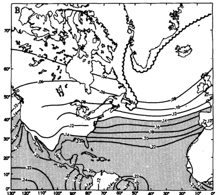
FIGURE 44.—Horizontal distribution of radiation imbalance at the earth's surface; (A) the distribution of the model (average of two hemispheric values) and (B) the distribution of the actual earth's surface, obtained by Budyko (1963); units, \text{ly min}^{-1} .
