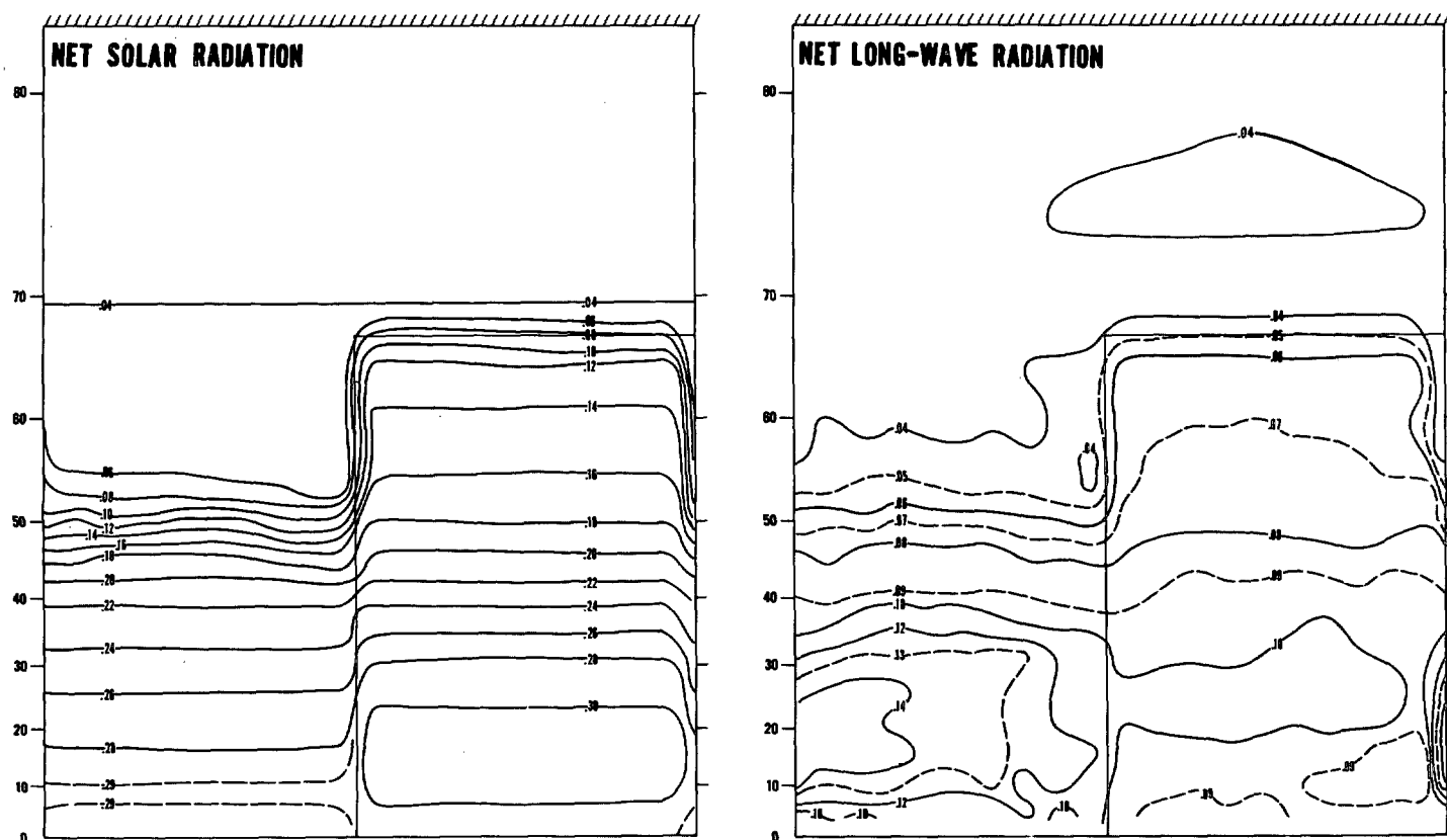
FIGURE 42.—Horizontal distributions of net downward solar radiation and of net upward long-wave radiation at the earth's surface of the model (average of two hemispheric values). Units, \text{ly min}^{-1} .
