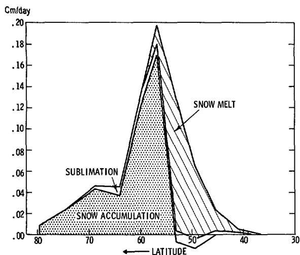
FIGURE 27.—Latitudinal distribution of the zonal mean snow budget on the continent of the model. The values of the two hemispheres are averaged. The negative rate of accumulation around latitude 50^\circ indicates the decrease of snow depth during the period of time averaging.
