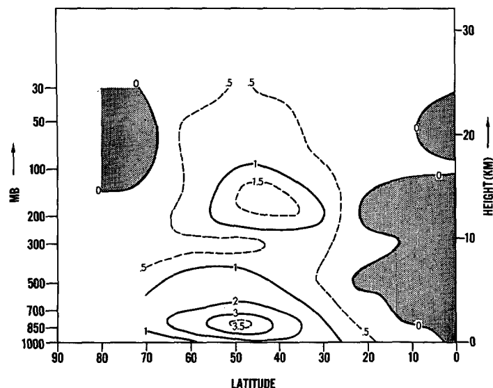
FIGURE 41.—Latitude-height distribution of poleward transport of heat in the actual atmosphere (Peixoto, 1958); units, 10^{17} joules \text{mb}^{-1} \text{day}^{-1} .
