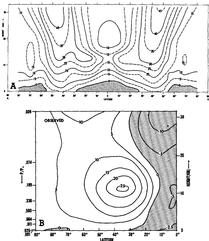
FIGURE 10.—(A) latitude-height distribution of the zonal mean of the zonal wind in the model atmosphere in units of \text{m sec}^{-1} ; the region of easterlies is shaded; (B) observed latitude-height distribution of the zonal mean of the zonal wind ( \text{m sec}^{-1} ) compiled from Rasmusson and Oort (1970), Oort (1964), and Batten (1964); the region of easterlies is shaded.
