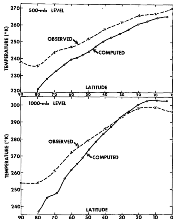
FIGURE 6.—Latitude distributions of zonal mean temperature at 500-mb and 1,000-mb levels. Solid and dashed lines indicate the computed and observed distributions, respectively. The computed distributions are obtained by taking the average of values of the two hemispheres. Observed distributions are based on the work of Peixoto (1960).
