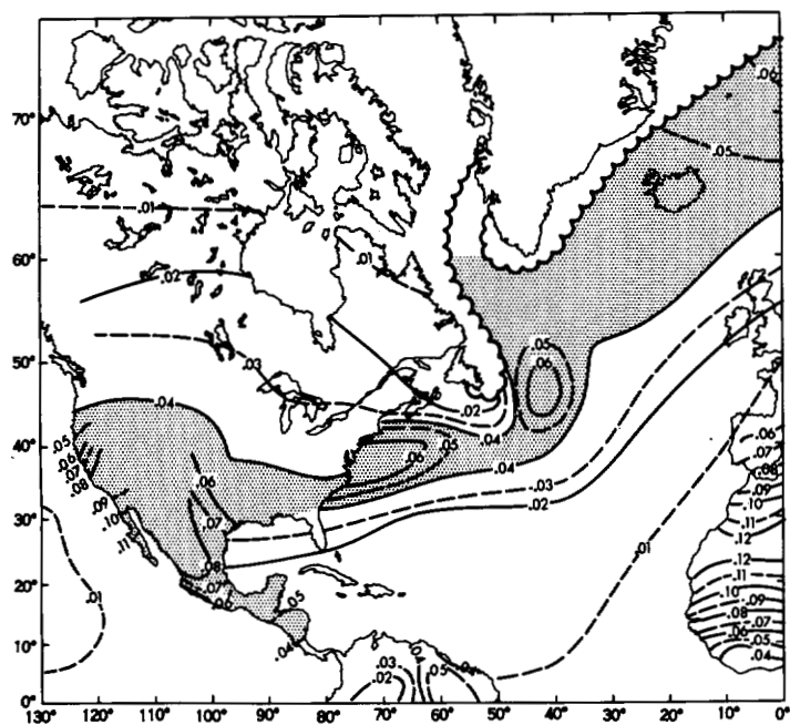
FIGURE 48.—Horizontal distribution of the turbulent flux of sensible heat at the earth's surface, estimated by Budyko (1963); units, \text{ly min}^{-1} .
