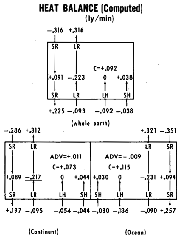
FIGURE 49.—Heat balance diagrams of the model. SR, solar radiation; LR, long-wave radiation; LH, latent heat flux; SH, sensible heat flux; C, heat of condensation; and ADV, advection.
