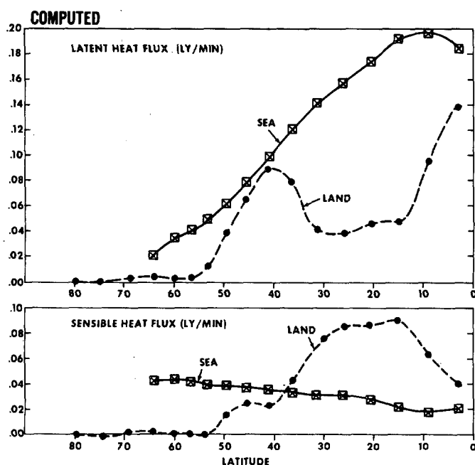
FIGURE 46.—Latitudinal distributions of zonal mean fluxes of sensible and latent heat for the continent and ocean separately. The distributions for the model are shown in the left diagrams (average of two hemispheric values), and the distributions of the actual earth's surface obtained by Budyko (1963) are shown in the right diagrams.
