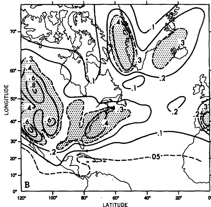
FIGURE 55.—(A) tracks of cyclones, generated in the latitude belt of 40^\circ \text{ N.} to 40^\circ \text{ S.} during 100 model days (243-343); solid and dashed lines indicate tracks in the Northern Hemisphere and Southern Hemisphere, respectively; (B) frequency of cyclogenesis, obtained by taking the average of summer and winter distributions compiled by Petterssen (1950).
