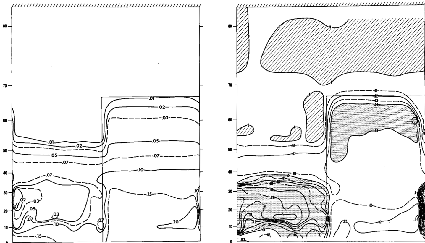
FIGURE 47.—Horizontal distribution of the turbulent flux of latent heat (left diagram) and sensible heat (right diagram), using the average of two hemispheric values; units, \text{ly min}^{-1} .
