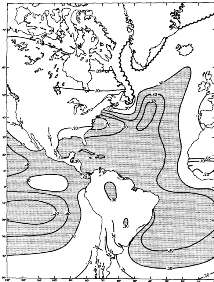
FIGURE 22.—Distribution of evaporation ( \text{cm day}^{-1} ) obtained by Budyko (1963).
