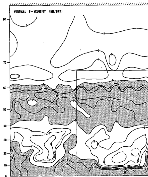
FIGURE 32.—Horizontal distribution of vertically integrated (pressure-weighted) vertical P -velocity of the model. The distributions of the two hemispheres are averaged.
