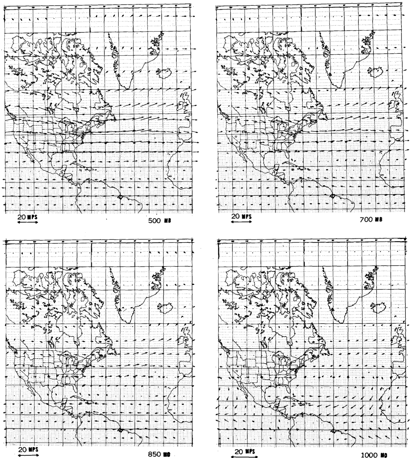
FIGURE 13.—Horizontal distributions of the vector wind at various pressure levels in the actual atmosphere. The length of the 20-m sec-vector wind is indicated near the lower left corner of each map. (Note that the unit length of the vector wind for the 1,000-mb-level map is different from the unit length of the other three maps.) These distributions were obtained by taking the average of a 5-yr period starting from May 1958 (Rasmusson and Oort, 1970).
