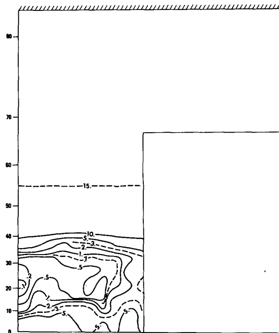
FIGURE 26.—Horizontal distribution of soil moisture (centimeters) of the model. The values of the two hemispheres are averaged.
