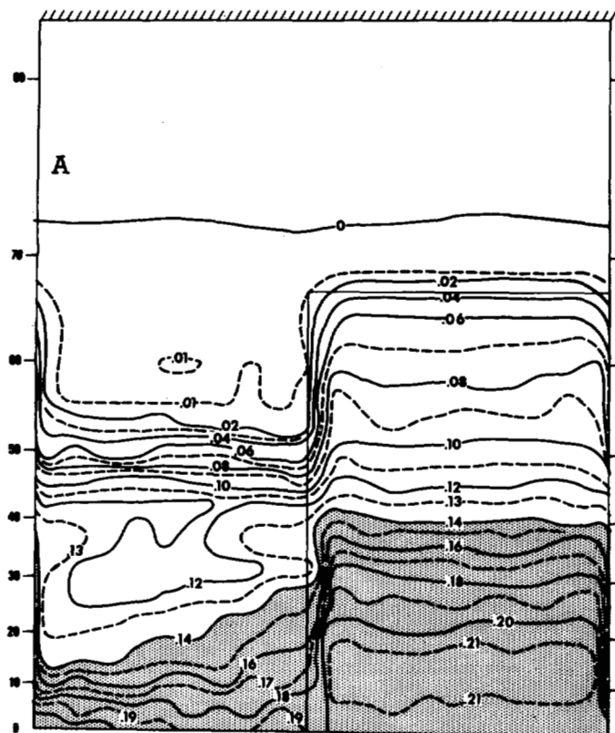
FIGURE 44.—Horizontal distribution of radiation imbalance at the earth's surface; (A) the distribution of the model (average of two hemispheric values) and (B) the distribution of the actual earth's surface, obtained by Budyko (1963); units, \text{ly min}^{-1} .
