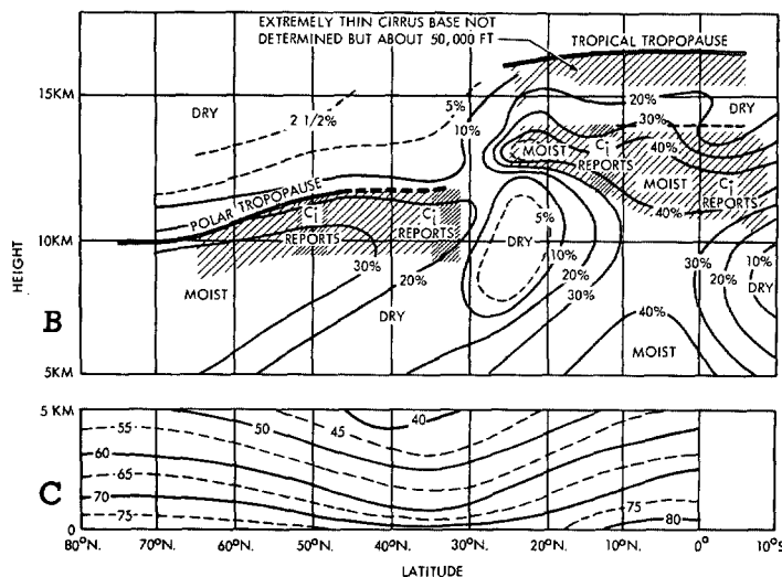
FIGURE 15.—(A) latitude-height distribution of zonal mean relative humidity in the model atmosphere (units, percent); (B) and (C) latitude-height distribution of mean relative humidities and cirrus distribution in the actual atmosphere (Northern Hemisphere) during the summer season; (B) from Murgatroyd (1960) and (C) from Telegadas and London (1954).
