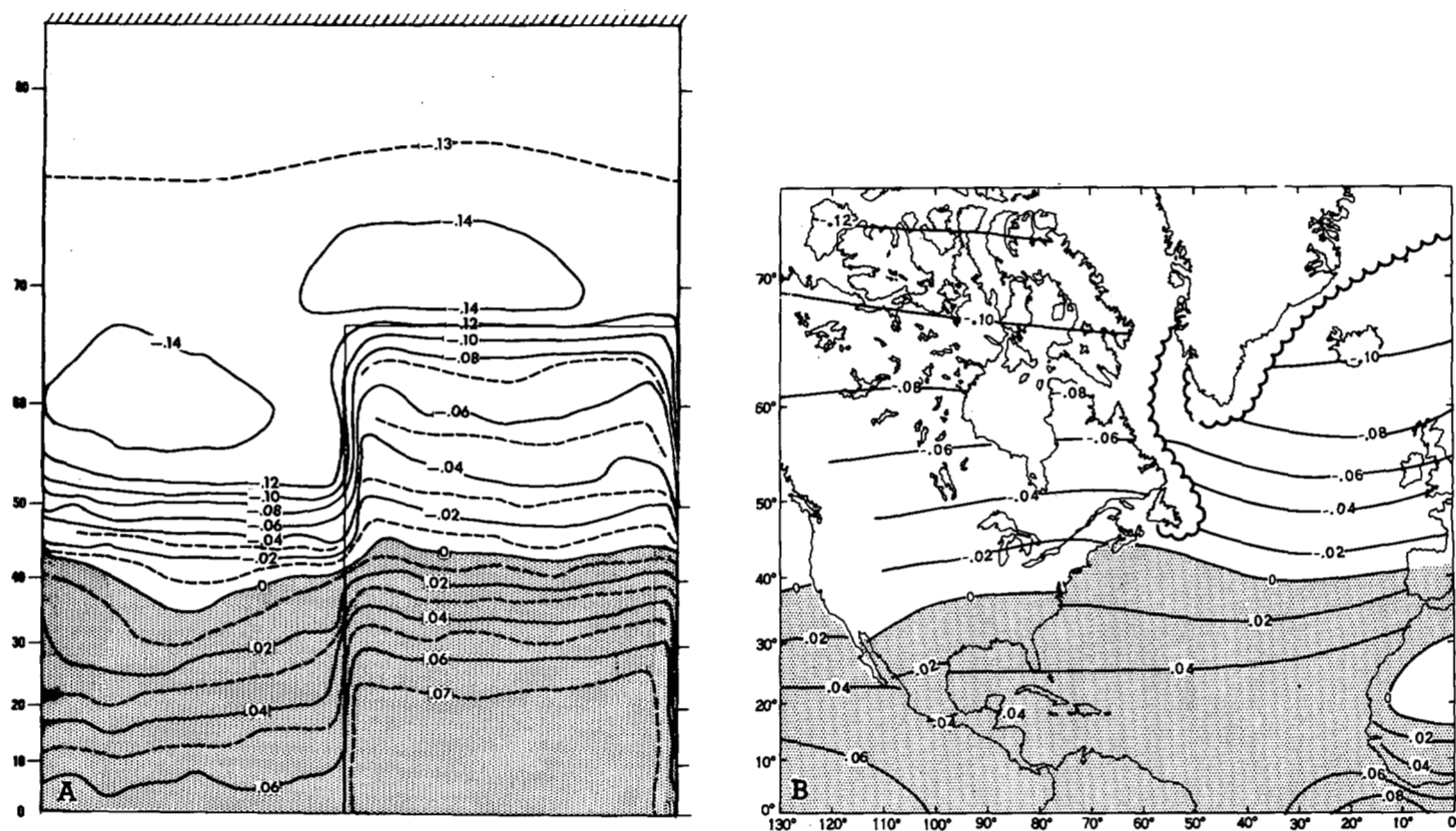
FIGURE 36.—Horizontal distribution of net downward radiation at the top of the atmosphere (radiation imbalance of the earth-atmosphere system); (A) distribution for the model (average distribution for the two hemispheres) and (B) distribution for the actual atmosphere, estimated by Budyko (1963); units, \text{ly min}^{-1} .
