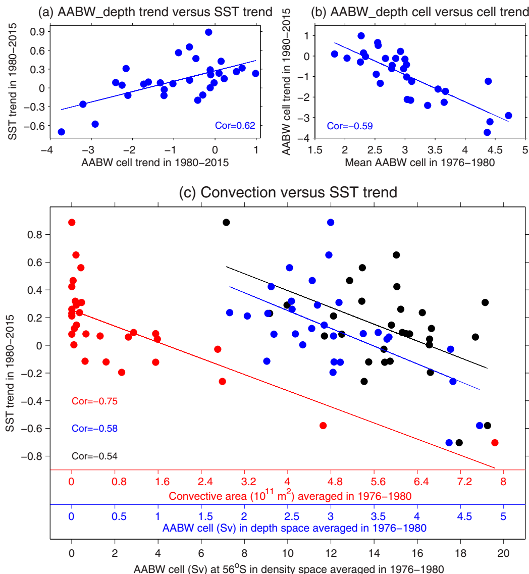
FIG. 5. (a) Scatterplot of annual mean AABW cell trend [in depth space; \text{Sv} (36 \text{ yr})^{-1} ] vs annual mean SST trend [ ^\circ\text{C} (36 \text{ yr})^{-1} ] in years 1980–2015 in SPEAR_LO_SSP585 large ensembles. (b) As in (a), but for the mean AABW cell strength averaged in years 1976–80 (Sv) vs the annual mean AABW cell trend [ \text{Sv} (36 \text{ yr})^{-1} ] in years 1980–2015. (c) As in (a), but for the mean SO convection strength averaged in 1976–80 (Sv) vs the annual mean SO SST trend in years 1980–2015 [ ^\circ\text{C} (36 \text{ yr})^{-1} ]. The SO convection strength is represented by the AABW cell index in depth space (blue dots; Sv), in density space (black dots; Sv) and convection area where the September MLD exceeds 2000m (red dots; 10^{11} \text{ m}^2 ). The lines in the panels denote the best linear fit according to least squares regression. The correlations are also shown in corners and all of them are significant at a 95% confidence level based on a Student's t test.
