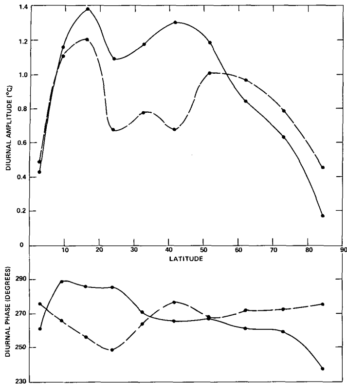
FIGURE 14.—The variation with latitude of the diurnal amplitude and phase of the temperature in the top level of model 4. Results for two longitudes 180^\circ apart are indicated by the full and dashed lines in the figure. The phases illustrated are for the time of the maximum.
