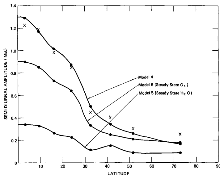
FIGURE 10.—The semidiurnal amplitudes of the surface pressure oscillations as a function of latitude are compared for models 4, 5, and 6. The difference between the amplitude of model 4 and that for either model 5 or model 6 indicates the contribution of water vapor or ozone respectively to the actual amplitude of the semidiurnal tide. The crosses give the values obtained by summing the amplitudes of models 5 and 6.
