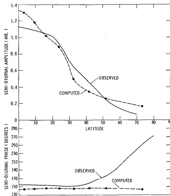
FIGURE 7.—Comparison of the semidiurnal amplitudes and phases of the surface pressure oscillation as a function of latitude for model 4 and observed values given by Haurwitz [6]. The computed values are the average of results at two longitudes 180^\circ apart. The phases illustrated are for the time of the maximum.
