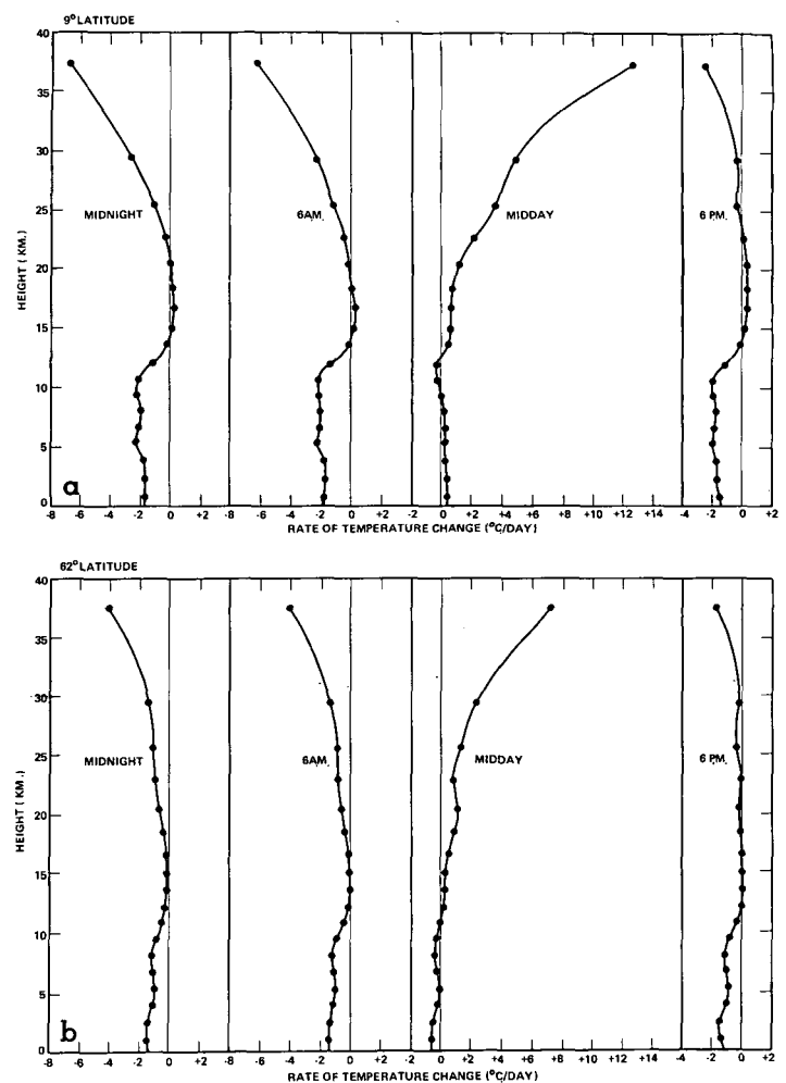
FIGURE 16.—(a) The net radiative temperature tendency for 9^\circ lat. is given as a function of height for four different times of the day. (b) Similar results for 62^\circ lat. are given. All results are for model 1.
