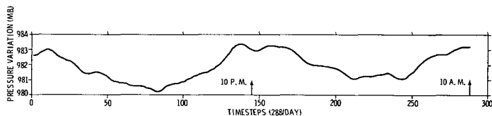
FIGURE 2.—The variation of the surface pressure oscillation in the Tropics for model 2 time averaged over a 3-day period. The surface temperature was fixed in this model.
