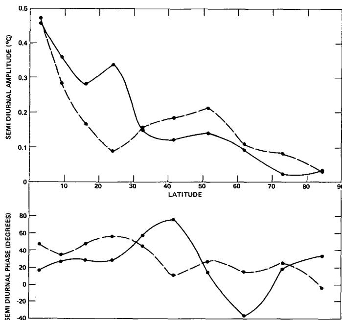
FIGURE 15.—The variation with latitude of the semidiurnal amplitude and phase of the temperature in the top level of model 4. Results for two longitudes 180^\circ apart are indicated by the full and dashed lines in the figure.
