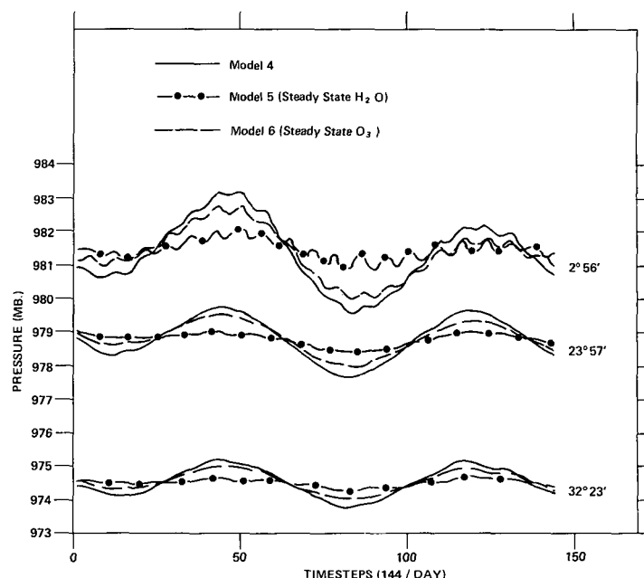
FIGURE 9.—A comparison of the surface pressure oscillations at selected latitudes for models 4, 5, and 6, illustrating the effects of removing the diurnal heating owing to the absorption of solar radiation by ozone or water vapor. Values shown have been time averaged over a 4-day period.
