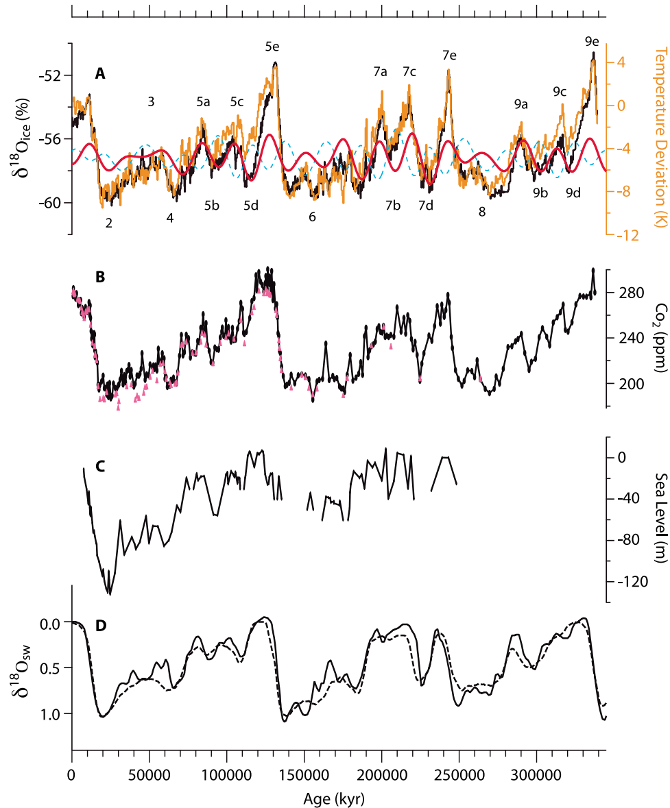
Figure 5. Comparison of (a and b) the temporal variability in Antarctic air temperature and atmospheric \text{CO}_2 with (c and d) sea level and northern ice volume over the last 340,000 years. Red curve in Figure 5a is the summer insolation at 65^\circ\text{N} . The warmest intervals in Antarctica tend to be front loaded within the first halves of the longer cycles while the second halves remain almost uniformly cold. Northern ice volume, in contrast, remains low during the first halves of the longer cycles and then builds up gradually through the second halves. Antarctic records are from Dome Fuji ice core [Kawamura et al. , 2007]. Sea level curve in Figure 5c is from Thompson and Goldstein [2005]. Ice volume curves in Figure 5d are from Waelbroeck et al. [2002] and Bintanja et al. [2005]. Reprinted by permission from Macmillan Publishers Ltd: Nature [Kawamura et al. , 2007, Figure 2], copyright 2007.
