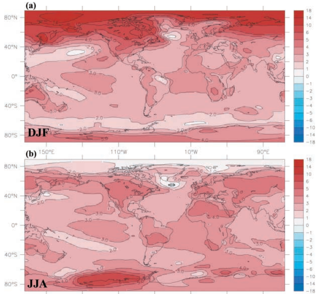
Fig. 16a, b. Spatial pattern of temperature changes for the period 2065–2089 relative to the control integration for the experiments described in Fig. 13. The map represents the ensemble mean of the GS_C_{1,2,3} experiments minus the corresponding sections of the control integrations. Positive values indicate that the GS_C ensemble mean is warmer than the control. a DJF b JJA
