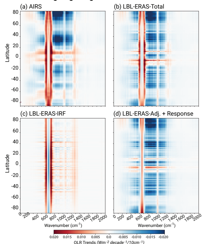
(a) AIRS satellite observations. (b) Simulation using ERA5 atmospheric conditions and GFDL's LBL-GRTCode radiation model. (c) Simulation showing only the instantaneous radiative forcing. (d) Simulation showing stratospheric and tropospheric adjustments along with the radiative response. Note that (c) and (d) together correspond to (b).
