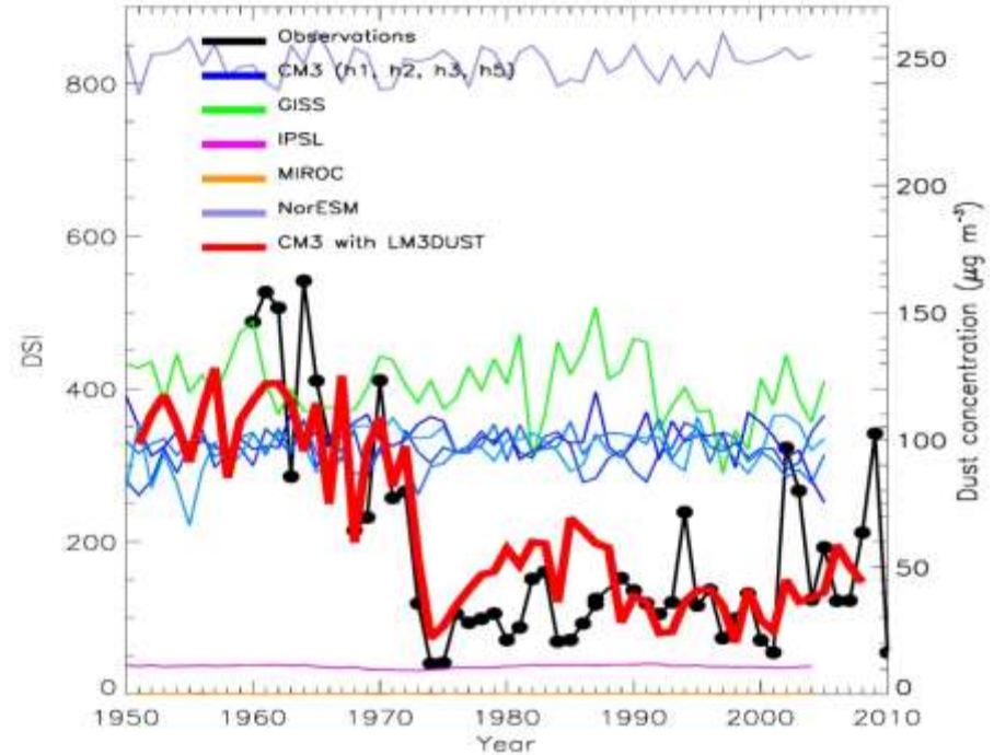
Dust Storm Index and simulated dust concentration Lake Eyre Basin (28.37S, 137.37E)
