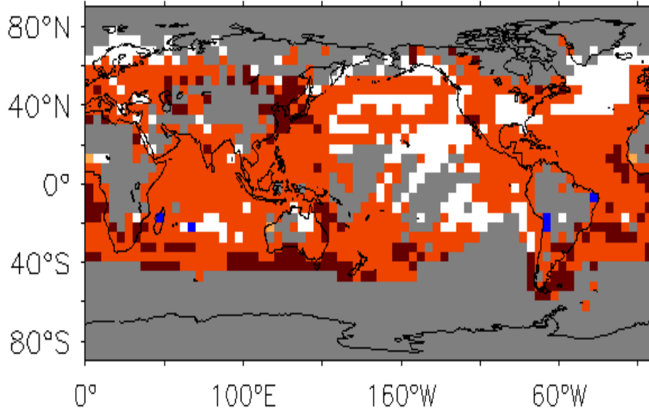
CMIP5 All-Forcing vs. Natural-Forcing assessment
