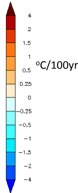
CMIP5 All-Forcing ensemble trend
