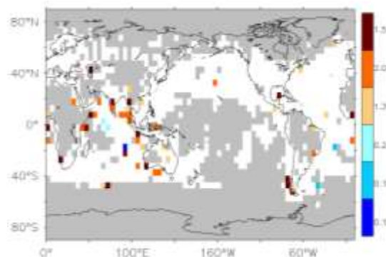
Dec.-Feb. 2013 seasonal extremes
