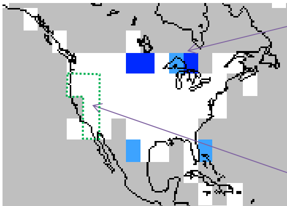
Annual 2013 Extremes - Precipitation
