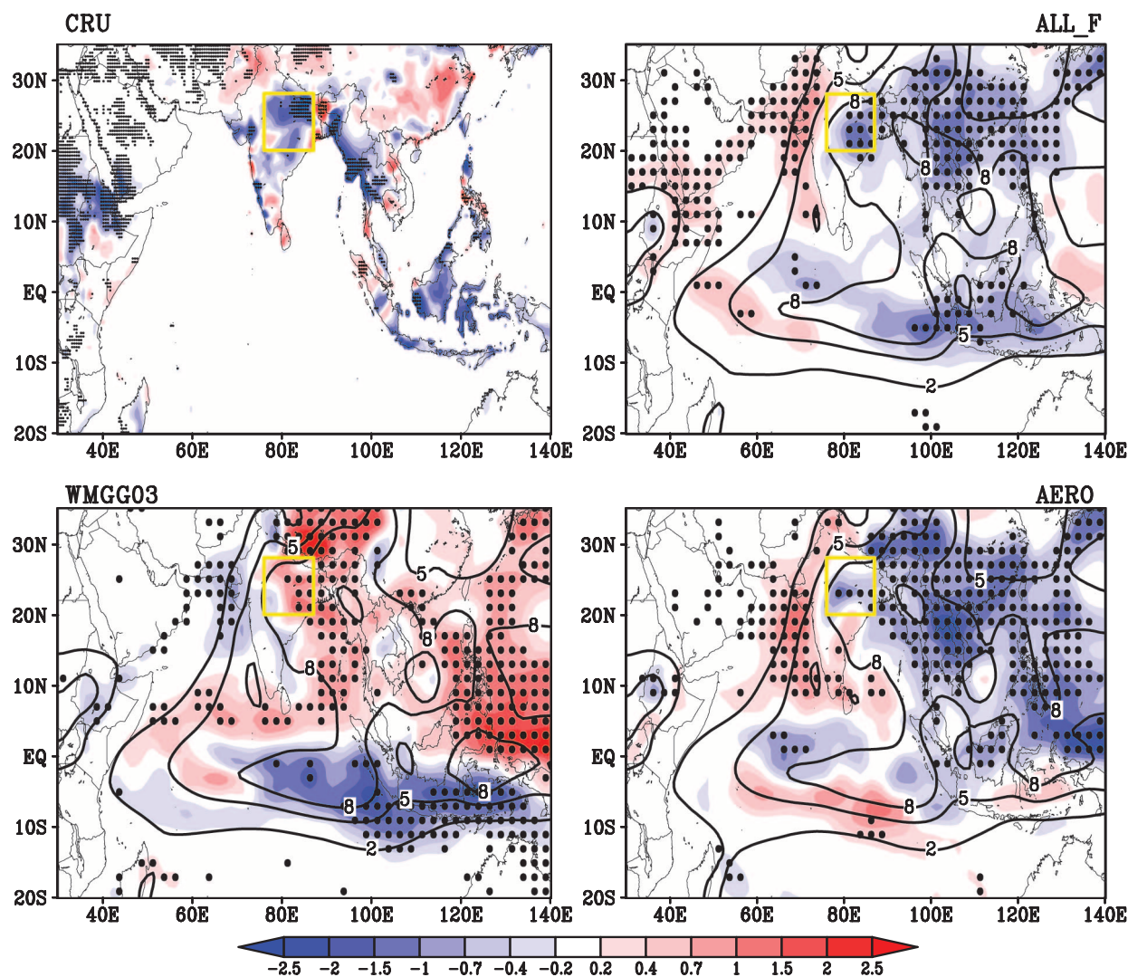
Fig. 2. Spatial patterns of the 1950–1999 least-squares linear trends of the June–September average precipitation [ \text{mm day}^{-1} ( 50 \text{ years}^{-1} )] according to the CRU TS 3.0 observational data set and the ensemble-mean all-forcing (ALL_F), aerosol-only (AERO), greenhouse gases and ozone-only (WMGG03) CM3 historical integrations. The black dots mark the grid points
